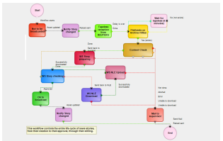
Nunzio workflow
